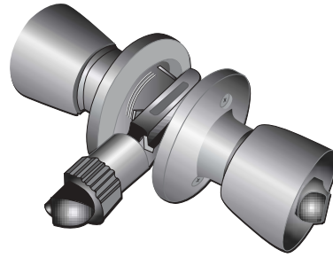
B-2939 BRASS PASSAGE DOOR LOCK B-2940 BRASS PRIVACY DOOR LOCK
