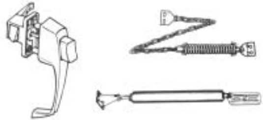
B-2961-K STORM DOOR HARDWARE KIT • A complete set containing all necessary hardware for installing a wood or metal combination door, 1" to 1-1/4" thick.
